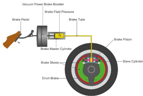
Hydraulic Drum Brake System
