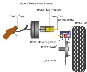
Hydraulic Disc Brake System
